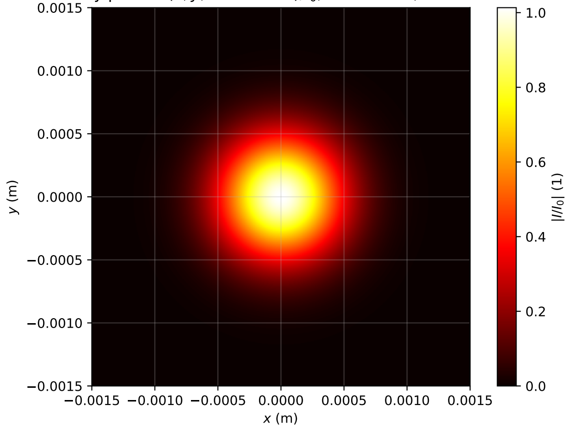
Intensity profile I(x, y, z = 0.239m)/I_0 , Pin=0.5Pcr, artificial time
